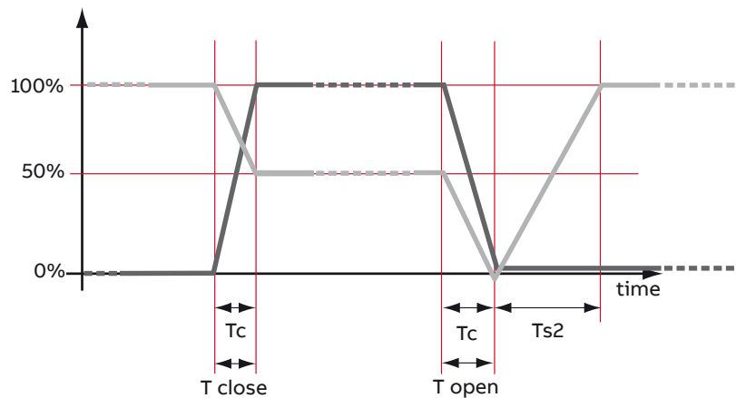
DIAGRAM OF 2S - DOUBLE SPRING OPERATING MECHANISM OPERATION
