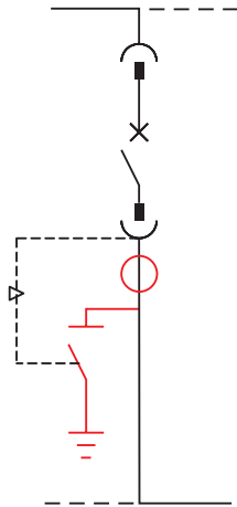
WBS: coupler unit
