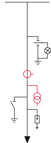
BME: direct feeder with measurement and busbar earthing
