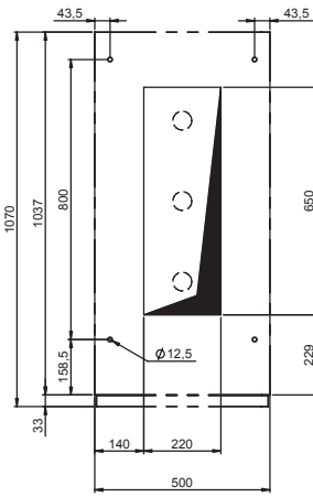
Units 500 mm wide
