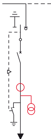
SBC: feeder with circuit-breaker and switch-disconnector
