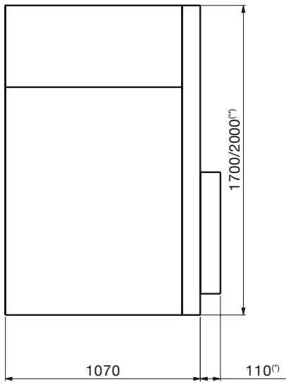
Side view IAC A-F 16 kA 1s, basic solution
