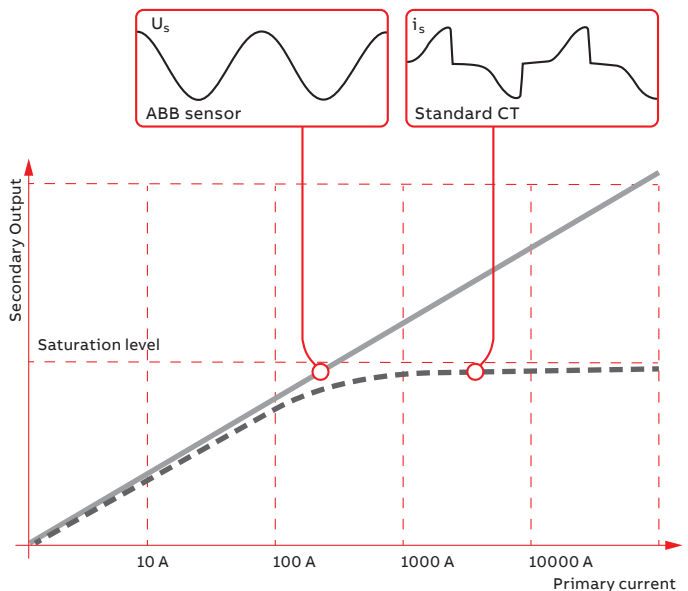
— Linearity of the ABB sensors and comparison with the wave shape of the output signals of a conventional saturation current
