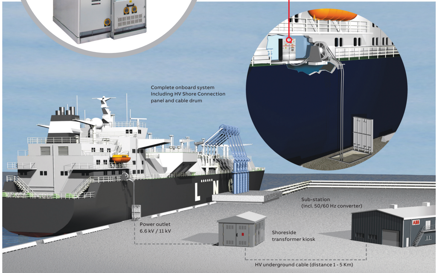
The picture illustrates the version with bottom cable connection. An alternative version with frontal plug connection is also available.
