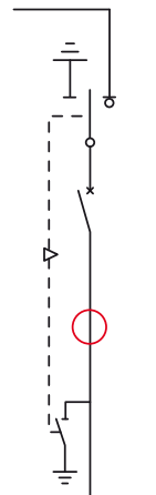
SBS: coupler with circuit-breaker and switch-disconnector
