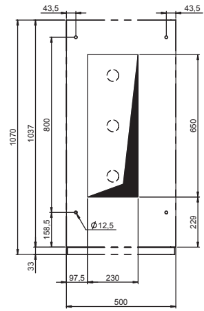
500 mm width for DRC unit
