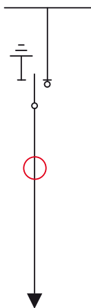
SDC: feeder with switch-disconnector
