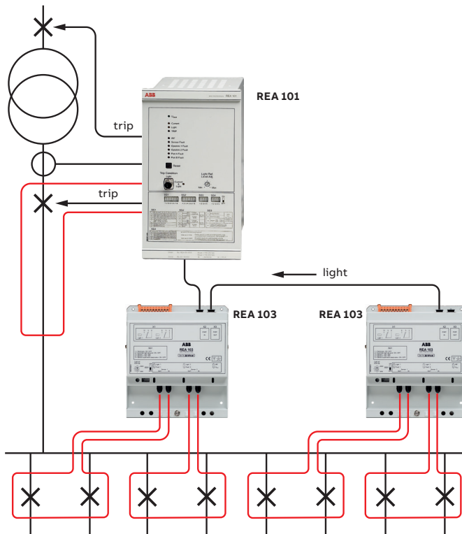
— Typical configuration with REA 101 and subunit 103
