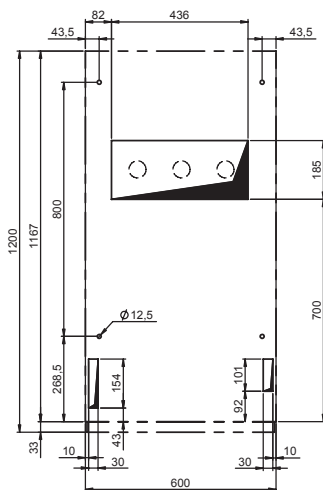
600 mm width for units with withdrawable circuit-breakers up to 17.5 kV WBS and BME without cable outlet
