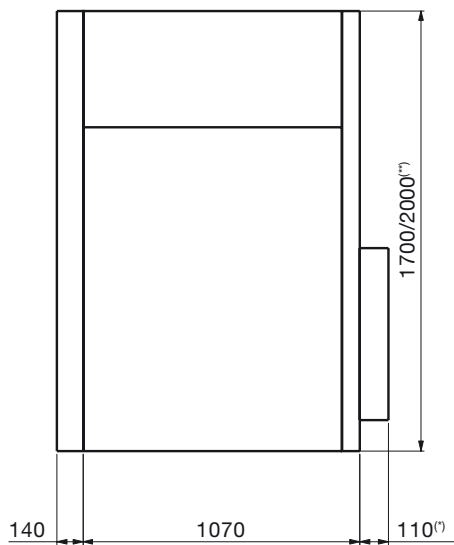
Side view IAC A-FLR 16 kA, with filters
