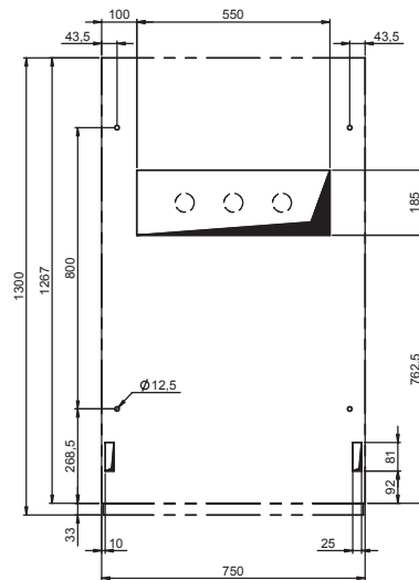
750 mm width for units with withdrawable circuit-breakers up to 24 kV WBS without cable outlet
