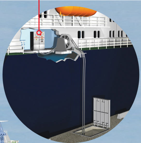
The picture illustrates the version with bottom cable connection. An alternative version with frontal plug connection is also available.
