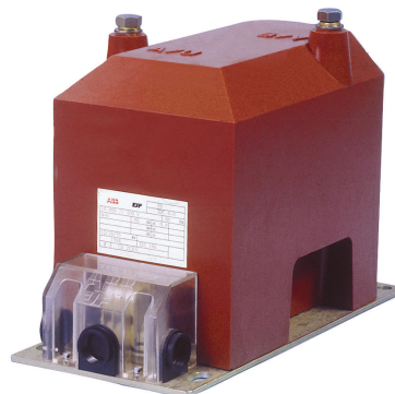
— Phase-to-phase VT – type TDC
