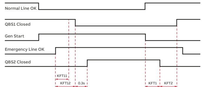
Diagram of ATS SDD switching times
