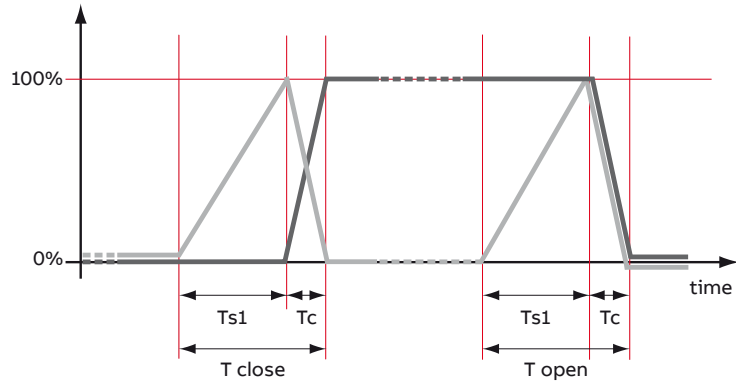
DIAGRAM OF 1S - SINGLE SPRING OPERATING MECHANISM OPERATION
