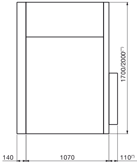
Side view IAC A-FLR 21 kA, with downward gas duct
