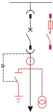
WBC: feeder unit
