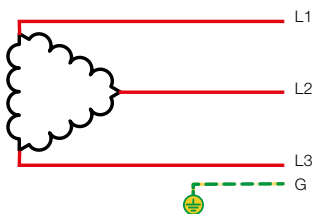
High-Leg Delta networks 240 / 1200 V HLD
