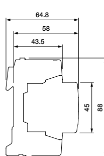
OVR T2 3L 40-400/690 P
